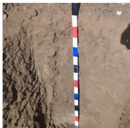
Figure 4. Representative soil profile for soil mapping unit-2.
